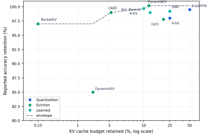
Fig. 4. Memory-accuracy frontier plotted from author-reported points (Table 5). Settings differ across papers, so positions are indicative, not a controlled comparison; the MBE harness (Section 10) produces the controlled version. Takeaway: accuracy holds remarkably flat until very aggressive budgets, where a sharp knee appears, and the position of that knee is what the right method, and a matched-budget comparison, decides.
